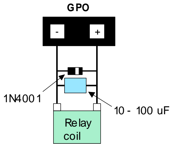
Figure 2-10 Clamping a Relay
