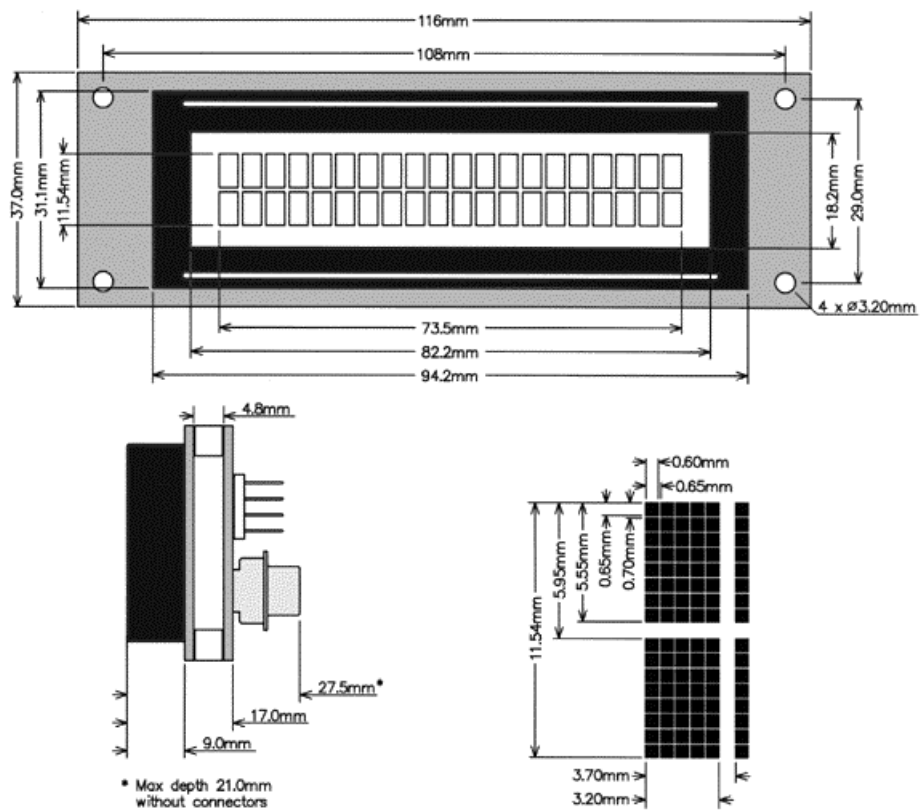
Figure 8-1 Physical Layout
