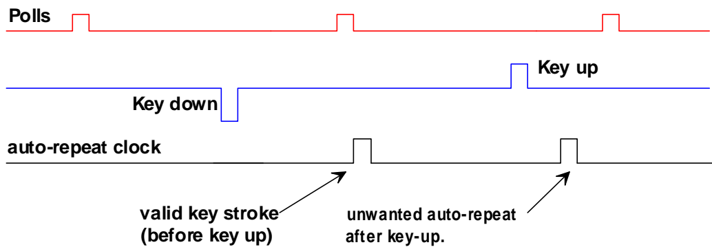
Figure 4-2 Poll timing
